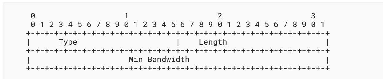
Figure 5: OSPF FAEMB Sub-TLV
